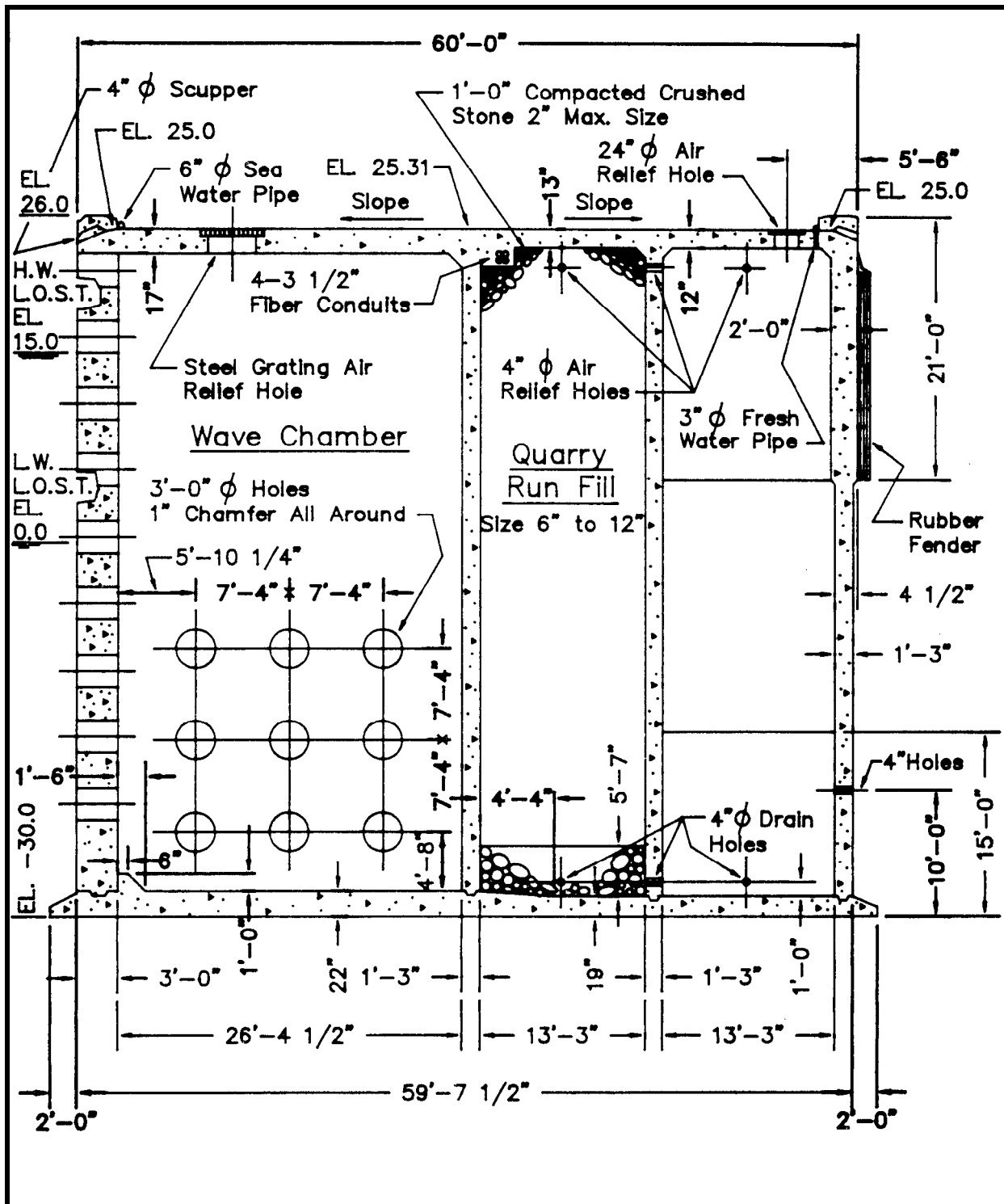
Figure 23 Typical Swiss-Cheese Perforated Breakwater Construction
