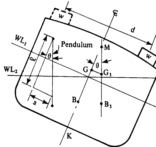
Figure 096-2-1. Effect of Weight(s) on Angle of List
